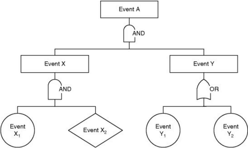
Figure 3.7 Example of an analytical tree.
