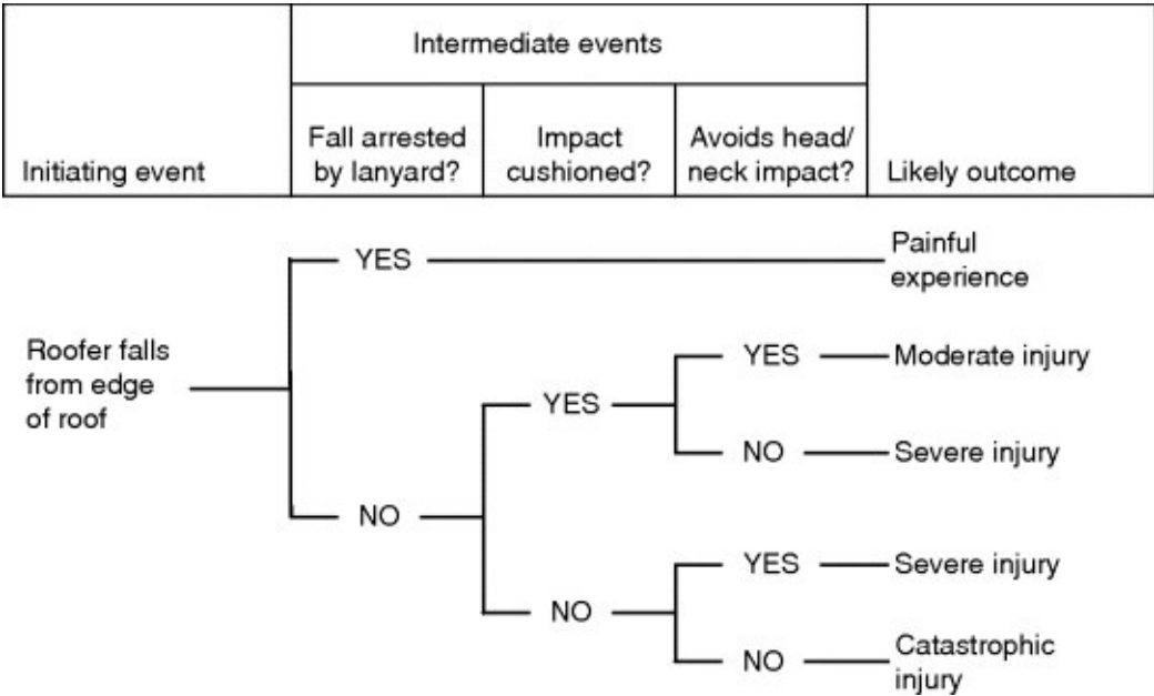
Figure 3.6 Example of an event tree.
