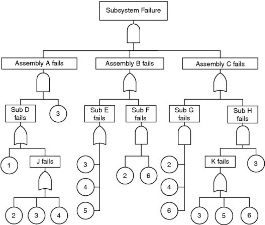
Figure 8.7 Fault tree illustrating a common-cause failure.
