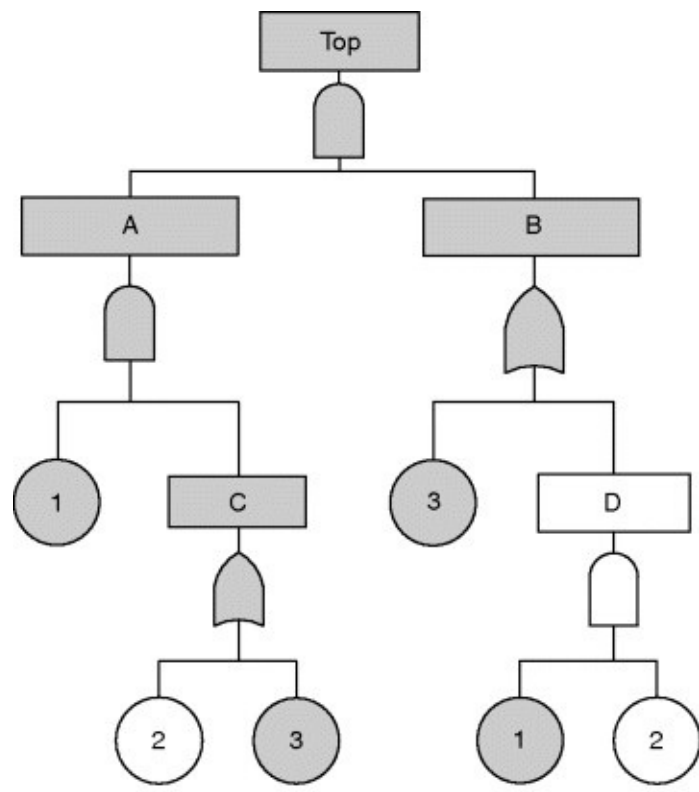
(a) Minimum cut set {1,3}
