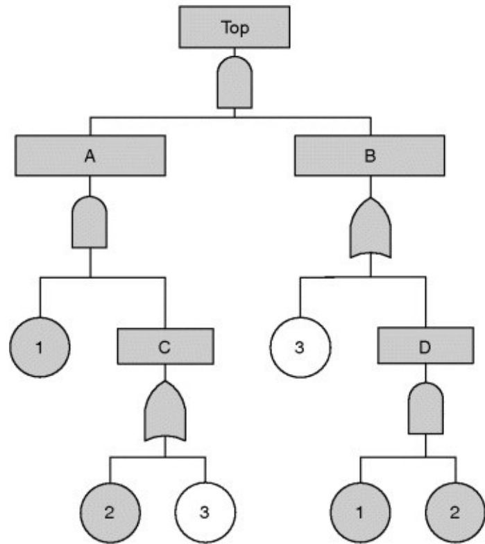
(b) Minimum cut set {1,2}
