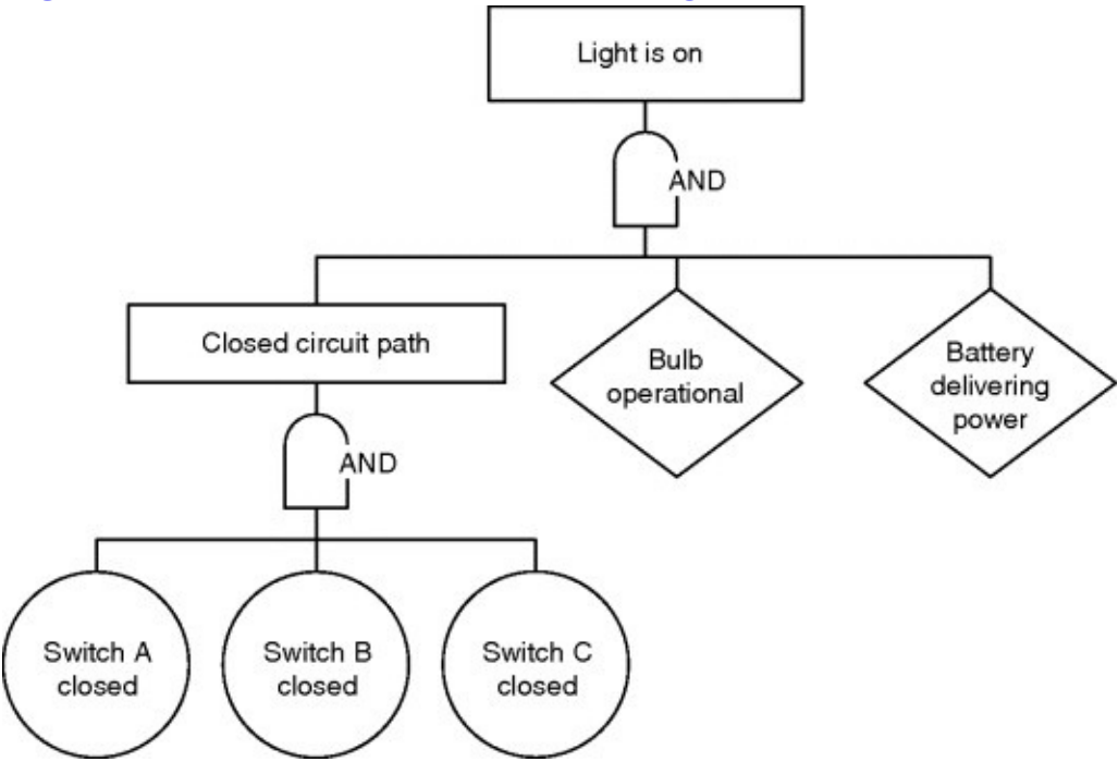
Figure 7.7 Success tree for circuit in Figure 7.4 .
