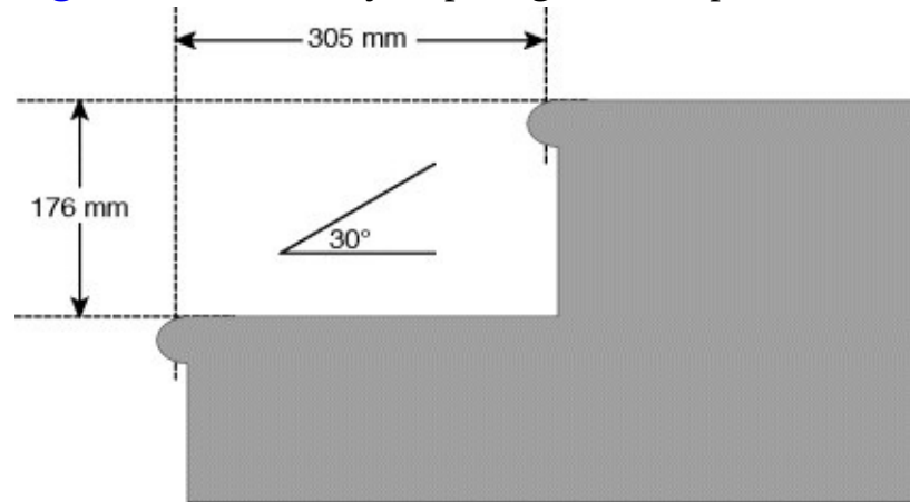
Figure 23.4 Stairway step height and depth measurement.
