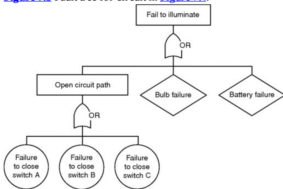
Figure 7.5 Fault tree for circuit in Figure 7.4 .
