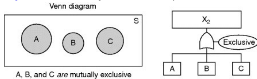
Figure 8.3 The OR gate for mutually exclusive events.
