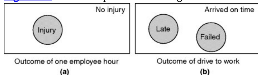
Figure 8.1 Two examples of Venn diagrams.
