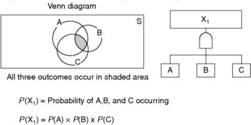
Figure 8.2 Understanding the AND gate.
